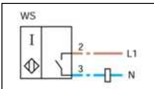
Normally Open (N/O)
