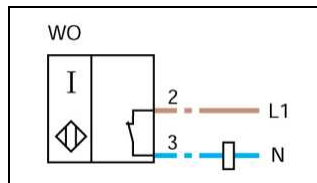
Normally Closed (N/C)
