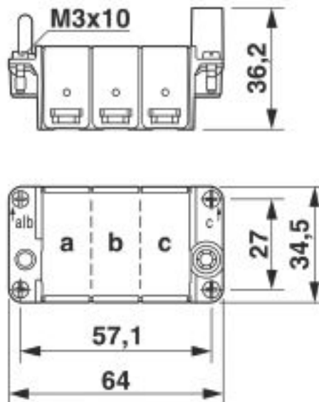
Dimensional drawing
