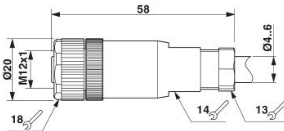
Dimensional drawing
