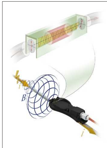
Fig. 34: Operating principle, Faraday effect
