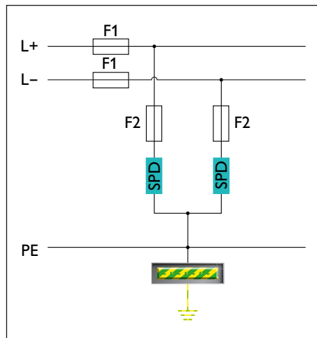
Fig. 66: 2+0 circuit for IT systems
