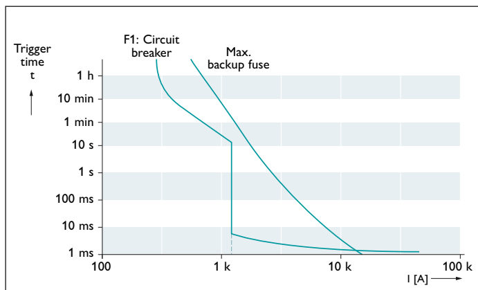
Fig. 56: Switching-off characteristics of a circuit breaker (F1) that is suited as an upstream overcurrent protective device for an SPD with maximum backup fuse of 315 A gG
