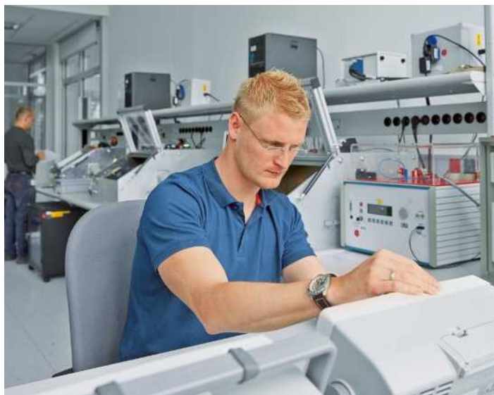
Fig. 26: Fully automated testing system for determining the overload and failure behavior of surge protective devices in accordance with IEC 61643-11 [6]
