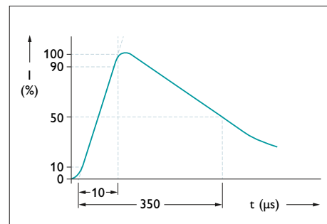
Fig. 21: Curve for a (10/350 μs) surge current pulse
