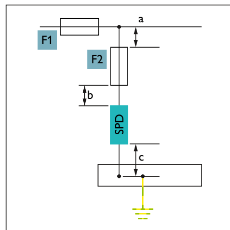
Fig. 53: Branch wiring
