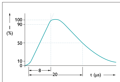
Fig. 19: Curve for a (8/20 μs) surge current pulse
