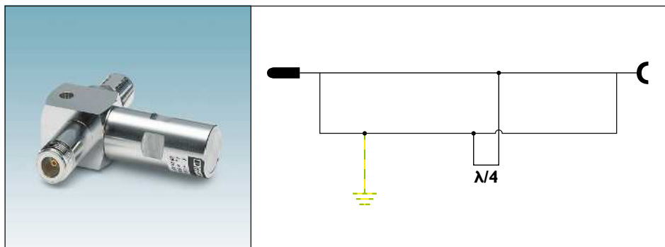
Fig. 103: CN-LAMBDA/4 - protective device with Lambda/4 technology
