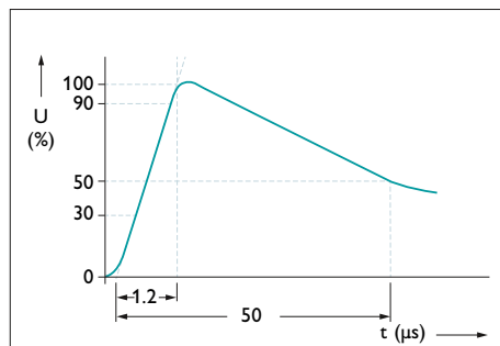
Fig. 20: Curve for a (1.2/50 μs) voltage surge pulse
