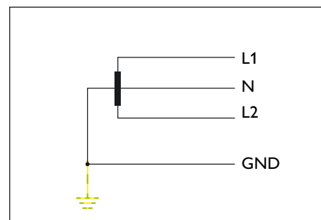
Fig. 50: Split-phase system
