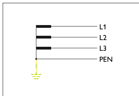
Fig. 45: TN-C system
