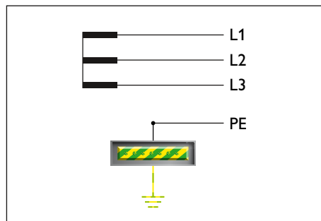
Fig. 47: IT system
