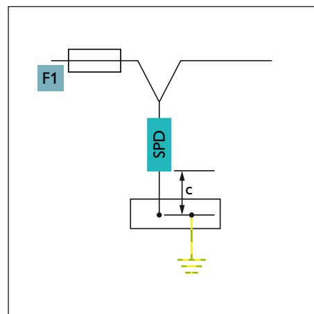
Fig. 54: V-wiring
