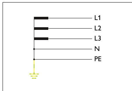
Fig. 44: TN-S system
