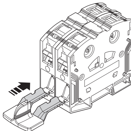
Figure 9 Insertion bridges
