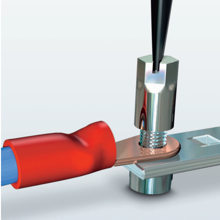
Figure 5 Bolt connection
