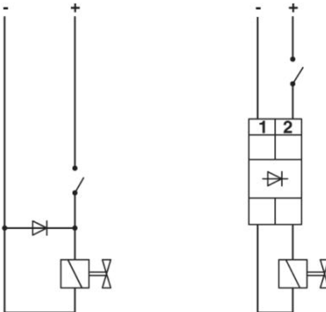
Circuit diagram
