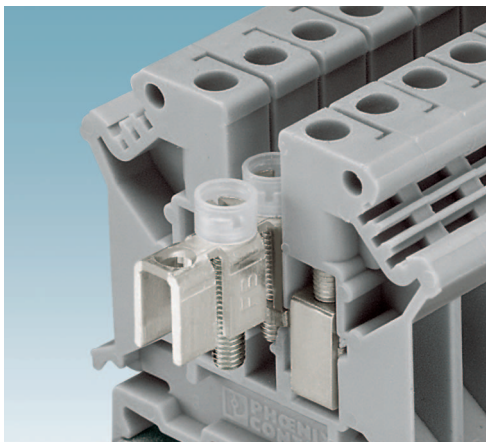
Figure 11 Fixed bridge
