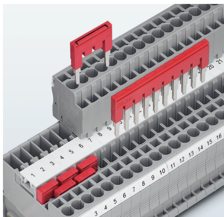
Figure 8 Plug-in bridges
