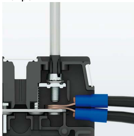
Figure 6 Barrier connection
