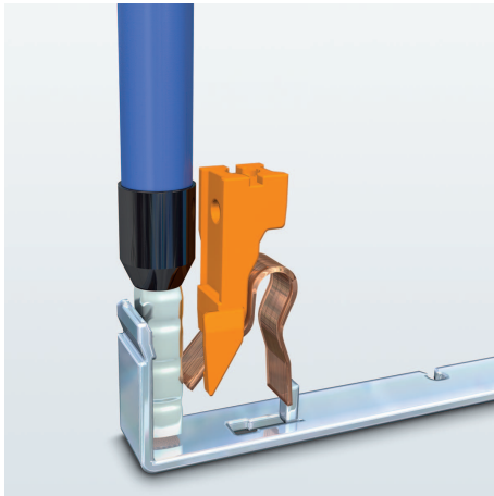
Figure 3 Push-in connection
