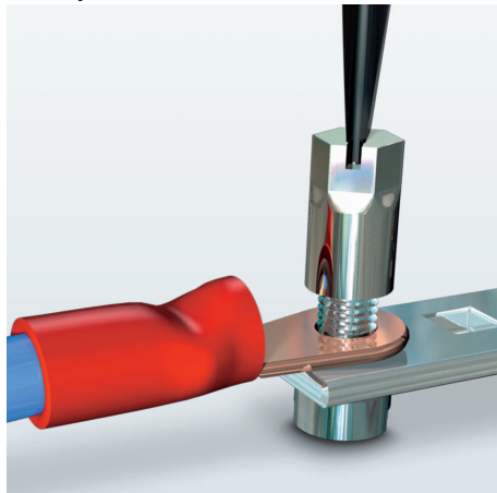
Figure 5 Bolt connection
