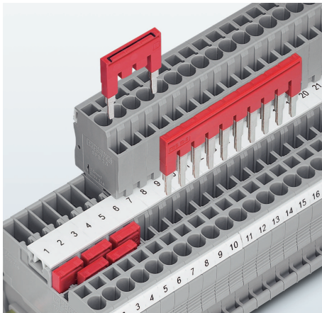
Figure 8 Plug-in bridges
