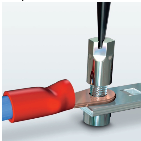
Figure 5 Bolt connection
