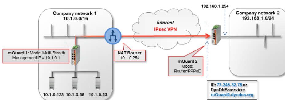
Figure 12-8 Connecting two networks via IPsec VPN (Multi Stealth <-> Router)
