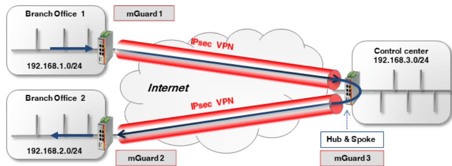
Figure 14-2 Hub and spoke via company control center (IPsec VPN)
