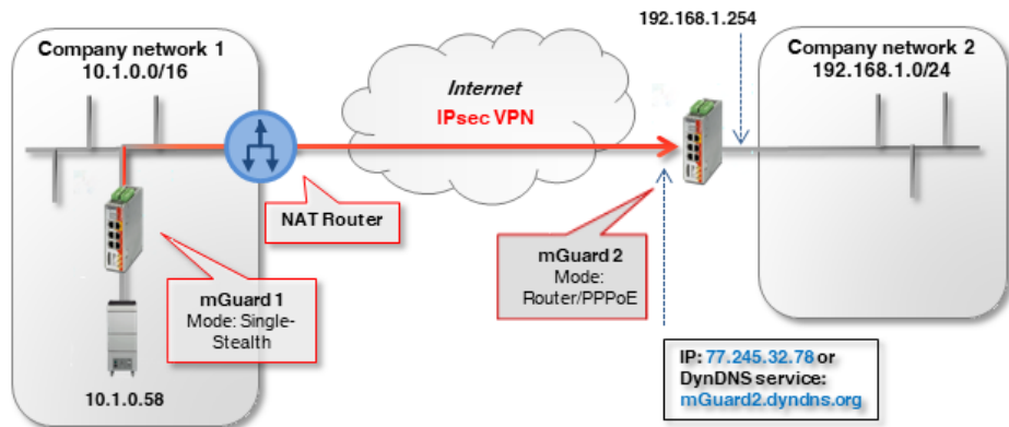
Figure 12-7 Connecting two networks via IPsec VPN ( Single Stealth <-> Router )
