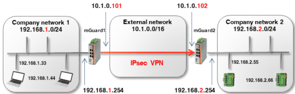
Figure 10-6 VPN connection between two networks with firewall
