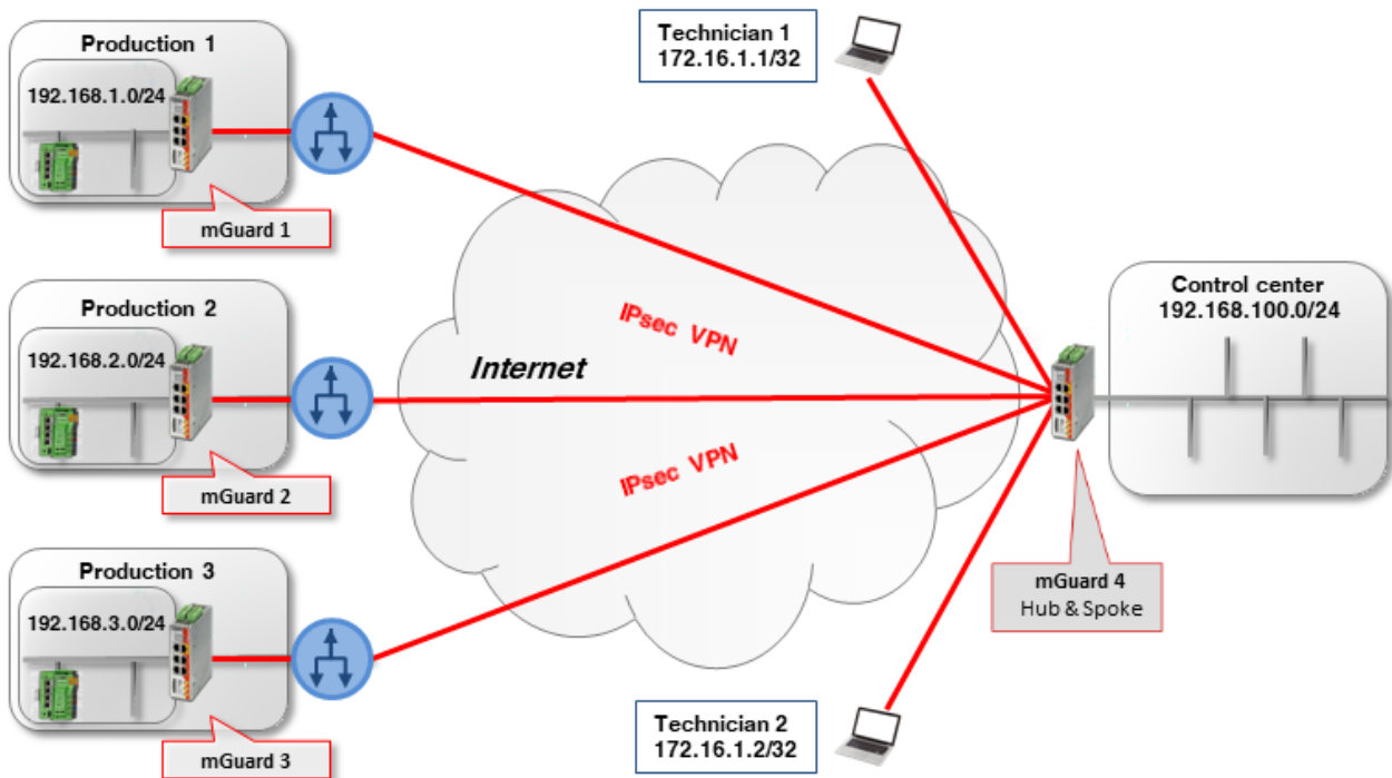
Figure 14-3 Remote maintenance via hub and spoke via the company control center (IPsec VPN)
