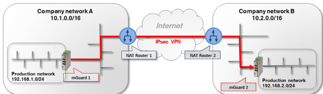
Figure 10-10 VPN initiator and VPN responder behind NAT routers
