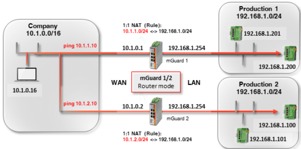
Figure 3-4 1:1 NAT rule: Accessing the entire production network from the company network
