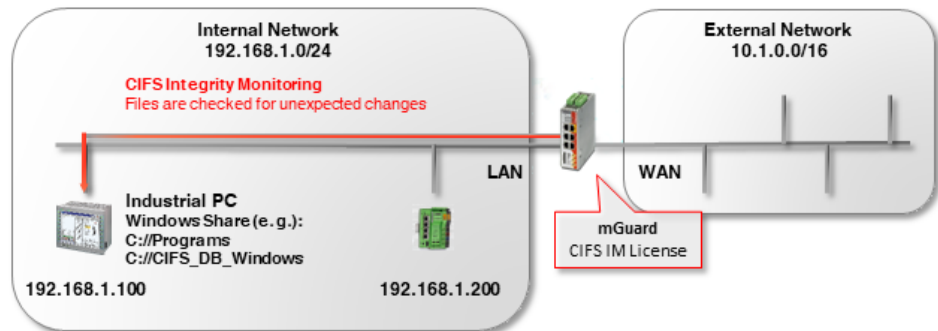
Figure 16-1 CIFS Integrity Monitoring – diagram
