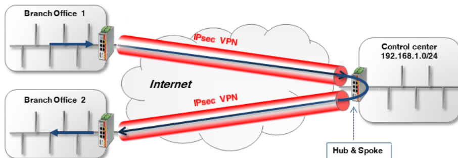
Figure 14-1 Hub and spoke via company control center (IPsec VPN)
