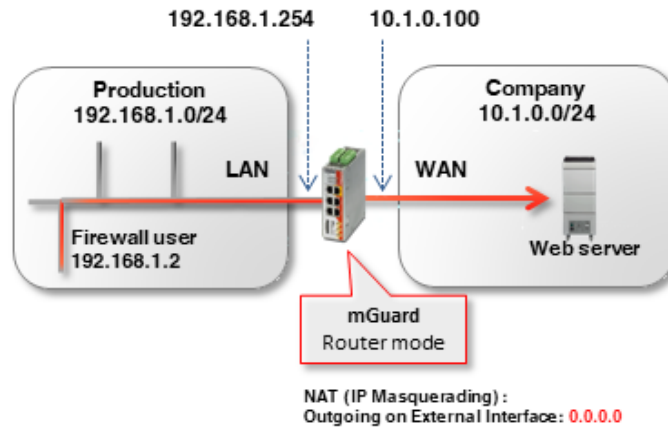
Figure 9-1 Firewall users with access rights to HTTP(S) web servers
