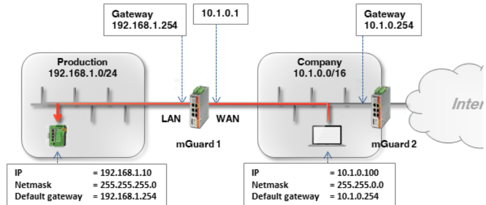
Figure 4-1 Client and mGuard router network settings
