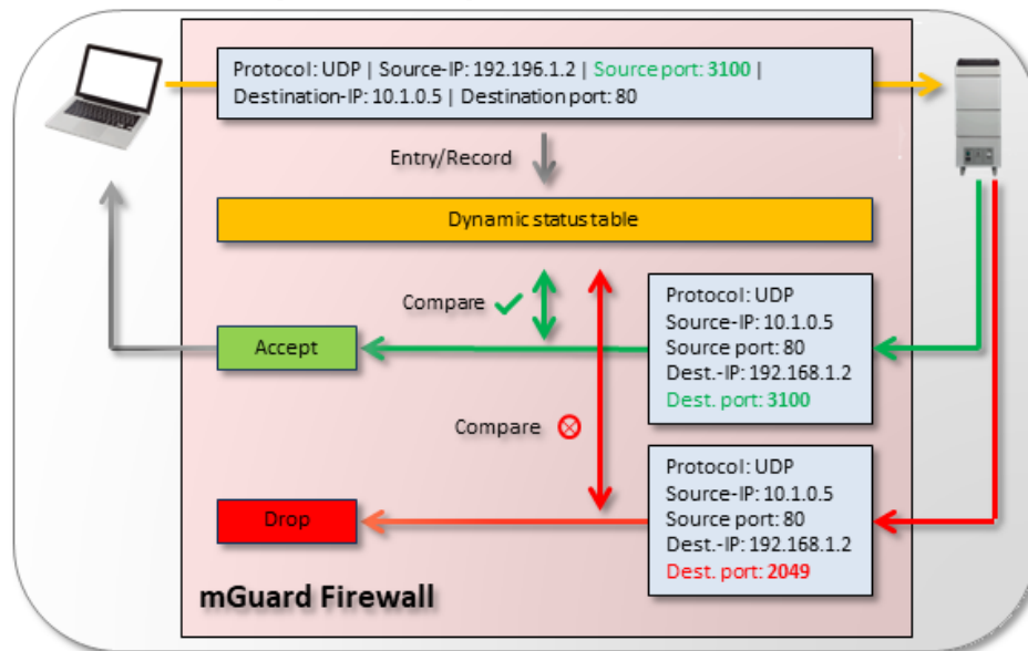
Figure 6-1 If incoming or outgoing packets pass the mGuard firewall (orange arrow), their properties (e.g. protocol, source IP/port, destination IP/port) are stored in a dynamic status table. The properties of the expected response packet are also stored in order that this also passes through the firewall. Response packets are then compared with the values in the status table. If the packets correspond to the dynamically entered values of the status table, they are accepted (green arrow). If they do not match, they are rejected (red arrow).
