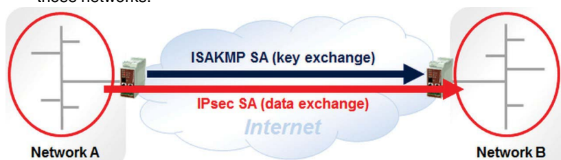
Figure 15-1 Establishment of the two phases of the VPN connection ( ISAKMP SA and IPSEC SA )
