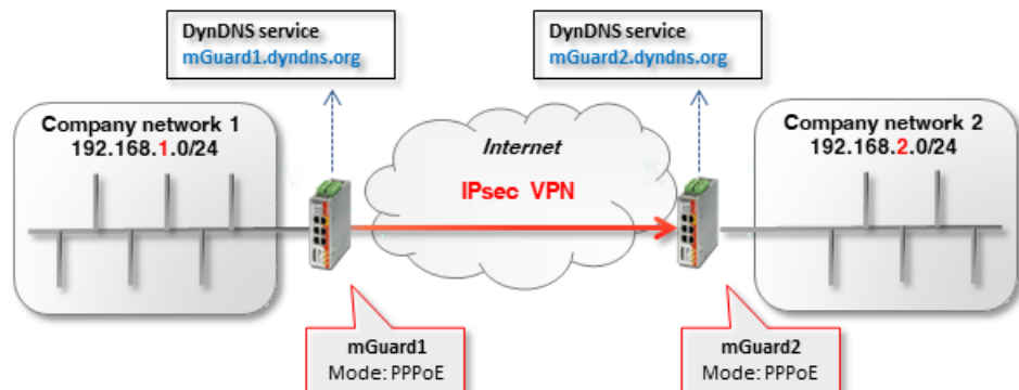
Figure 11-2 Determination of the host names for the mGuard devices using DynDNS. Because the VPN connection is initiated via mGuard 1 , this does not need a DynDNS address.
