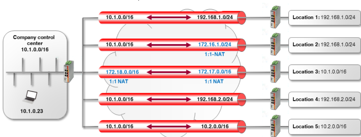
Figure 13-7 Transmission in both directions (local 1:1 NAT): the clients (e.g. PLCs) in the external networks can access the control center network via the VPN network, and vice versa.
