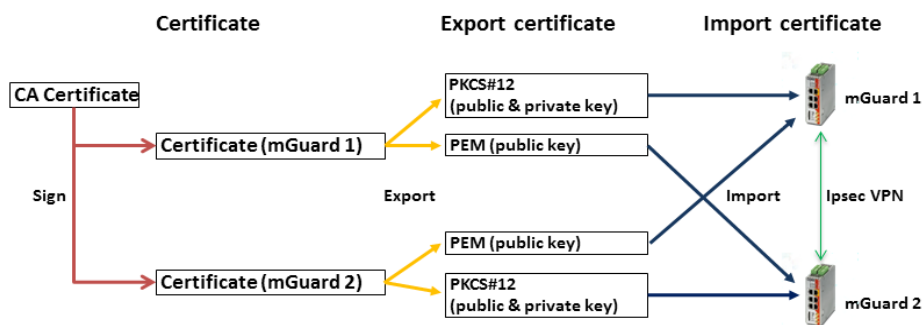
Figure 11-3 Participating certificates in an IPsec VPN connection
