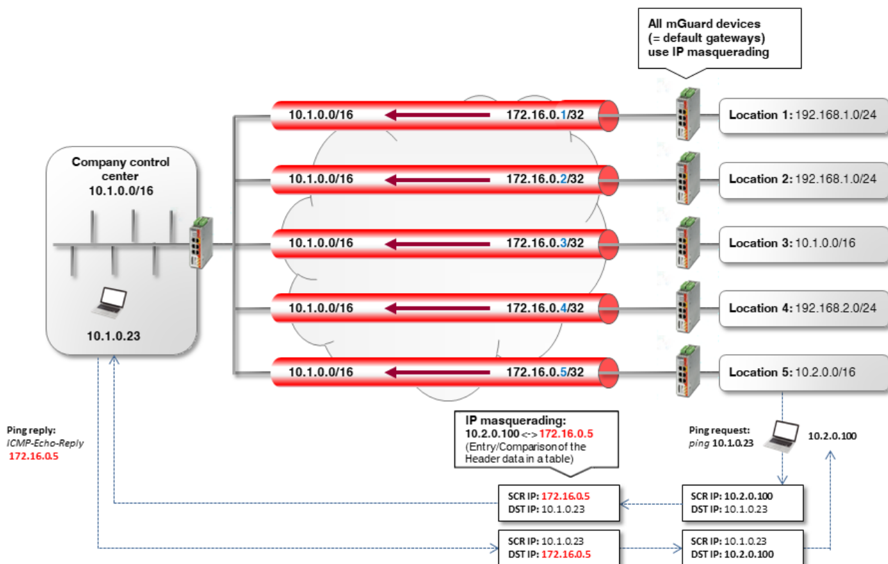
Figure 13-5 Transmission in just one direction (IP masquerading): clients (e.g. PLCs) in the external networks can send data to the control center via VPN. However, the control center cannot access the clients. The respective mGuard device is the default gateway of the internal client.
