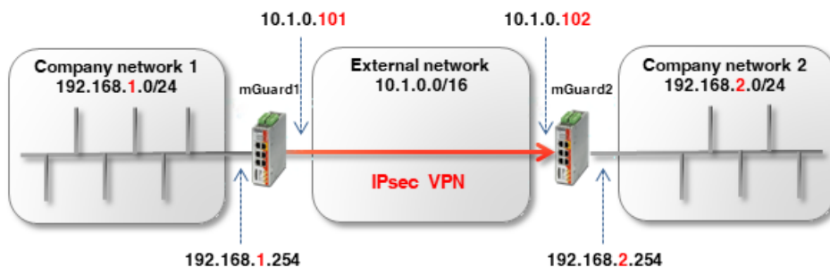
Figure 10-2 Connecting two networks via IPsec VPN
