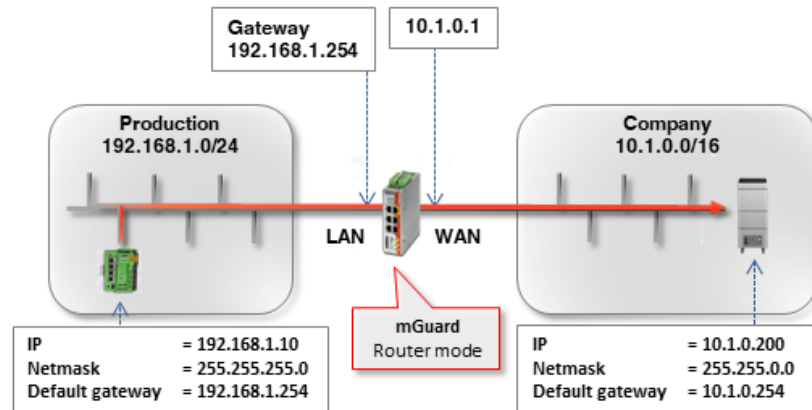
Figure 5-1 Client and mGuard router network settings
