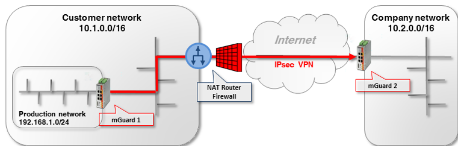
Figure 10-11 VPN initiator behind NAT router and firewall
