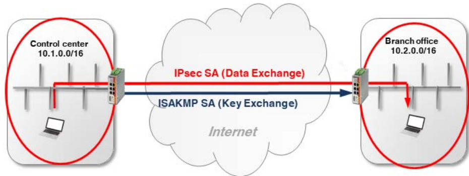
Figure 10-1 Setting up an IPsec connection (ISAKMP SA and IPsec SA)
