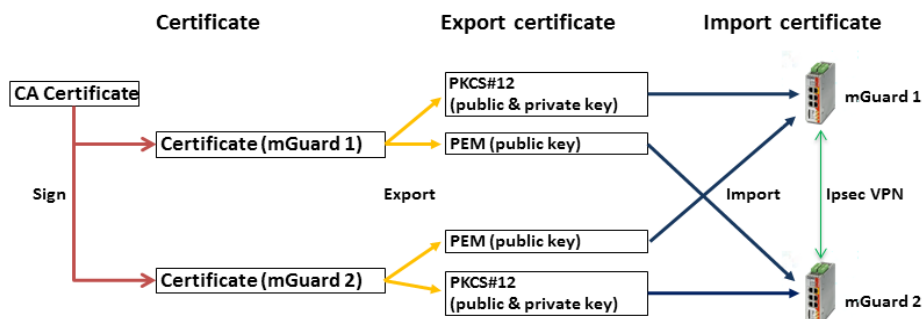
Figure 10-5 Necessary certificates in an IPsec VPN connection
