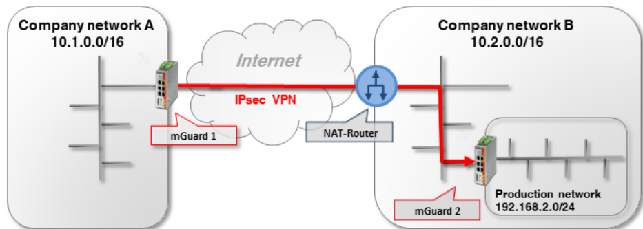
Figure 10-9 VPN responder behind NAT router
