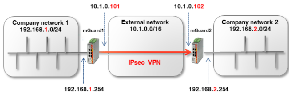
Figure 12-3 Connecting two networks via IPsec VPN
