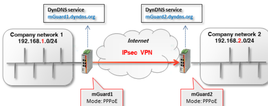
Figure 12-4 Connecting two networks via IPsec VPN ( Router/PPPoE <-> Router/PPPoE ). The host names for the mGuard devices are determined using DynDNS. (Because in this example the VPN connection is initiated by mGuard 1 , in principle it does not need a DynDNS address.)
