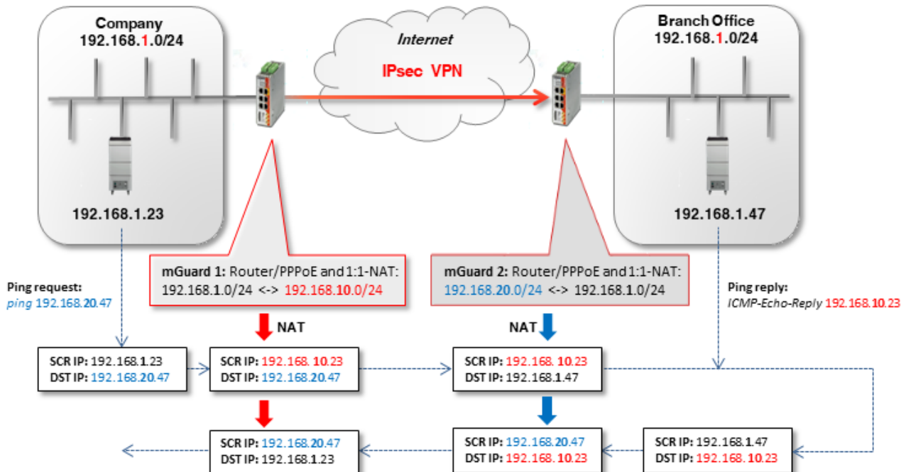
Figure 13-1 Same internal networks: ping request via a VPN tunnel using local 1:1 NAT
