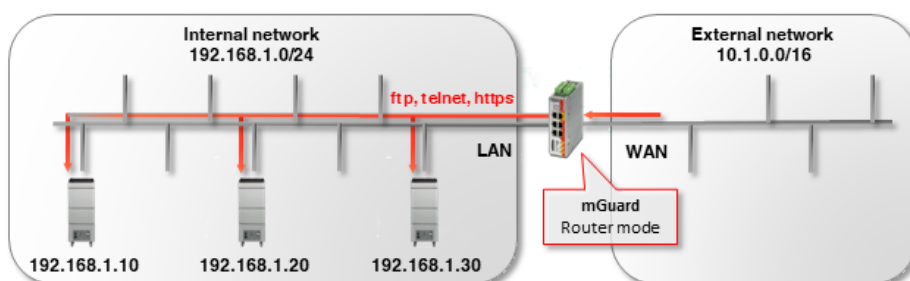
Figure 8-1 Allow access to special services on certain servers
