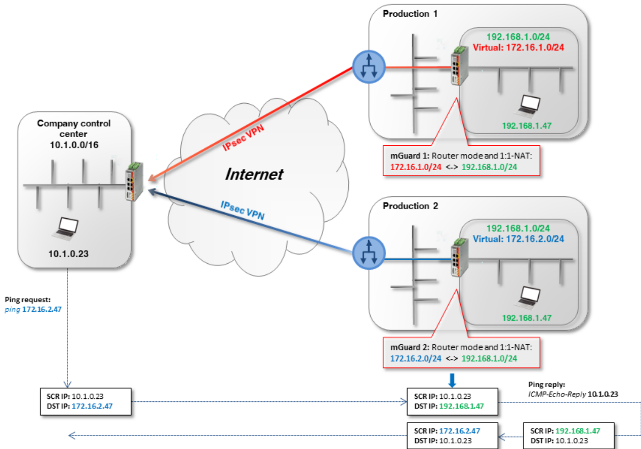
Figure 13-3 (Example mGuard 2) The same internal networks: ping request (to production 2) from the company control center via the VPN tunnel using local 1:1 NAT
