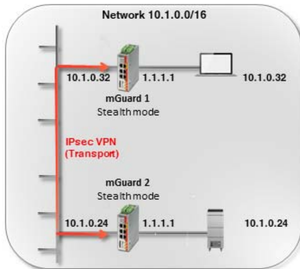
Figure 12-1 VPN transport connection in the Stealth network mode
