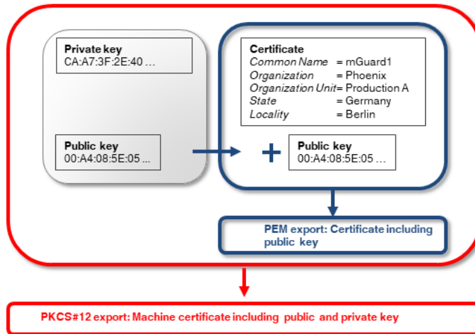
Figure 10-4 PEM and PKCS#12 exports of X.509 certificates with public or public and private keys
