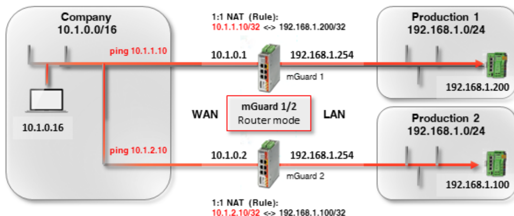
Figure 3-1 1:1 NAT rule: accessing individual IP addresses in the production network from the company network
