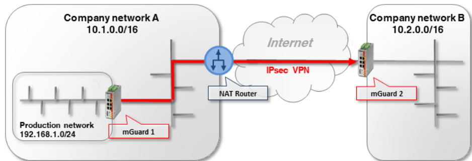
Figure 10-8 VPN initiator behind NAT router
