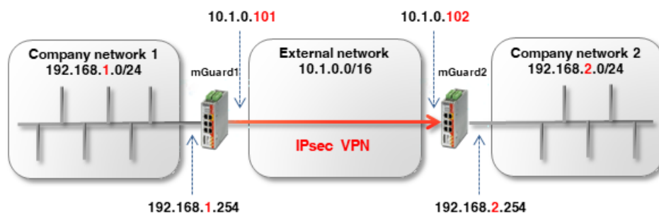
Figure 11-1 Connecting two networks via IPsec VPN
