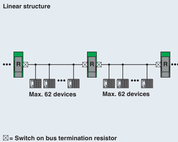
Figure 2 Line structure
