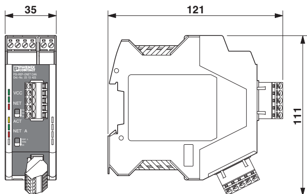
Figure 5 Housing dimensions
