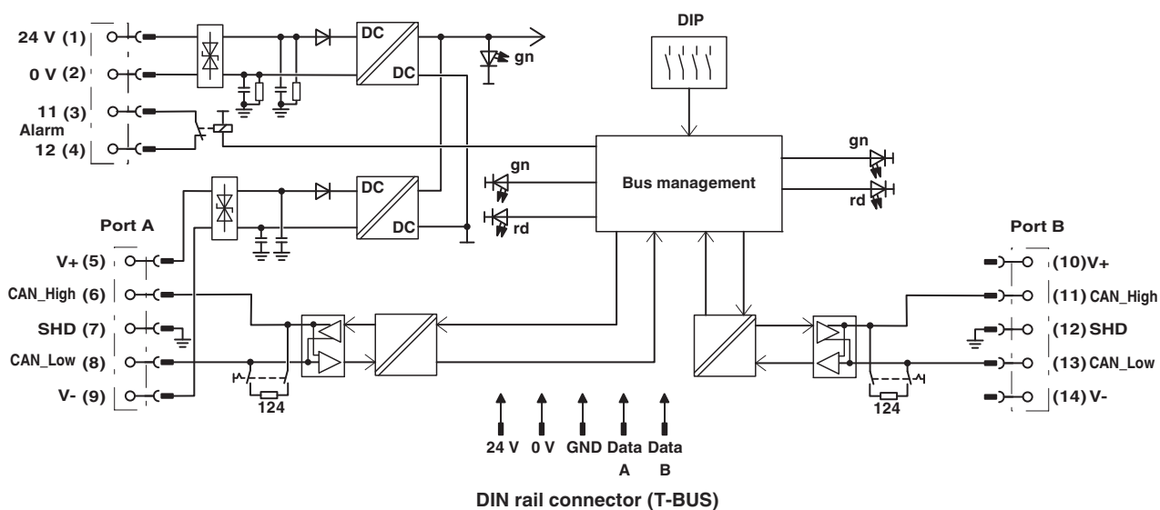
Figure 6 Block diagram
