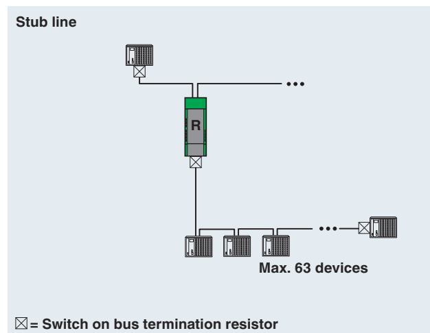
Figure 1 Branch line
