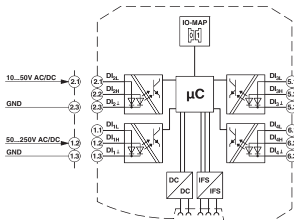
Figure 2 RAD-DI4-IFS basic circuit diagram
