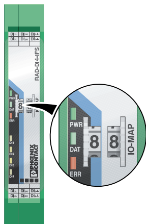
Figure 3 Thumb wheel
