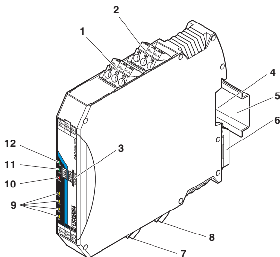
Figure 1 RAD-DI4-IFS
