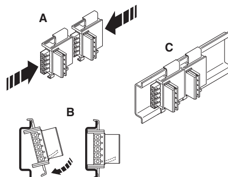
Figure 1 Installing the DIN rail connector
