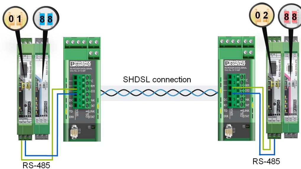
Figure 2 Schematic view
