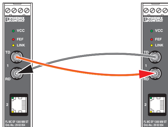
Figure 10 Signal direction for the fiber connection
