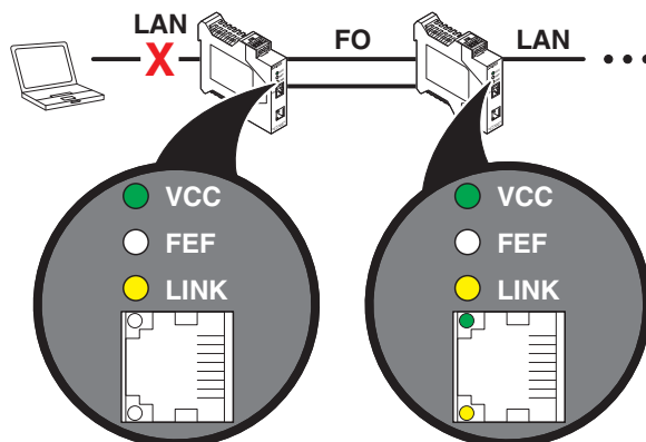
Figure 13 LAN fault with LFPT deactivated, local
