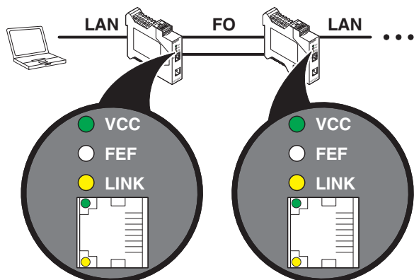
Figure 11 Diagnostics indicators in normal operation
