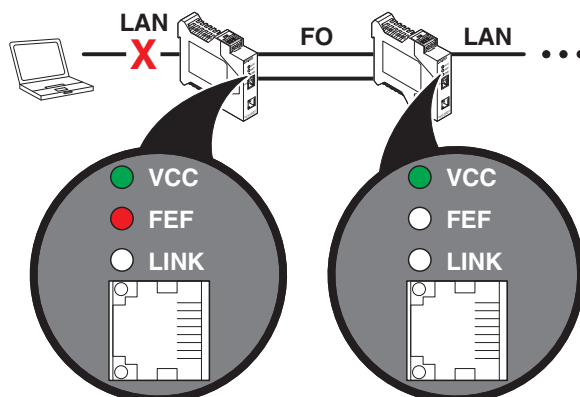
Figure 12 LAN fault with LFPT activated, global
