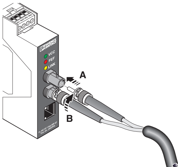
Figure 9 Connect B-FOC (ST ® ) plug
