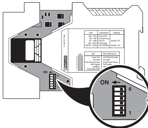
Figure 5 DIP switches
