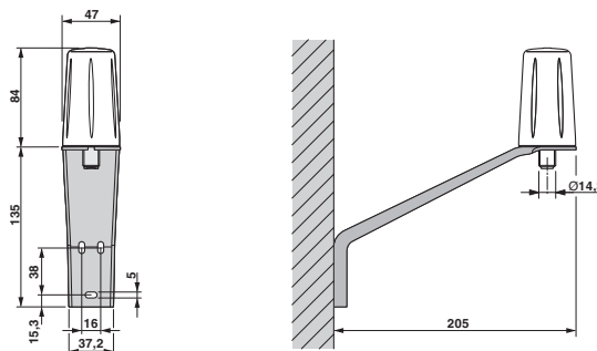
Figure 5 TC ANT MOBILE WALL 5M, wall mounting
