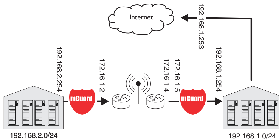
Figure 1-5 WLAN via VPN
