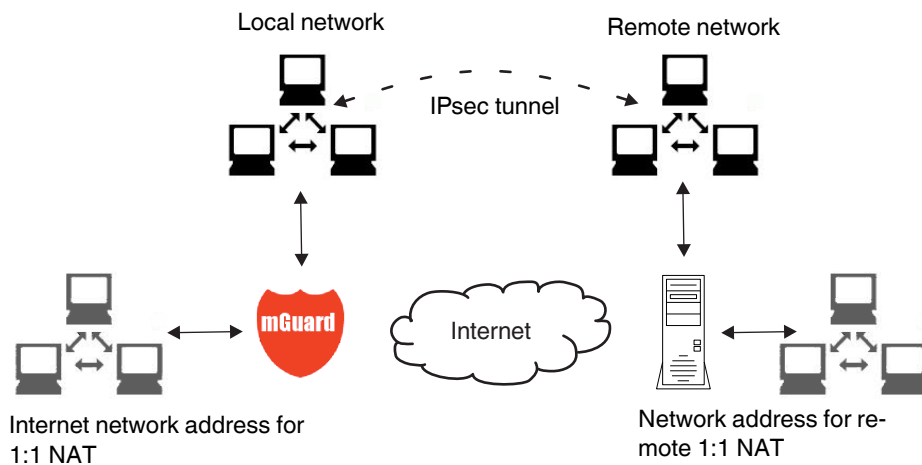
Figure 10-3 1:1 NAT
