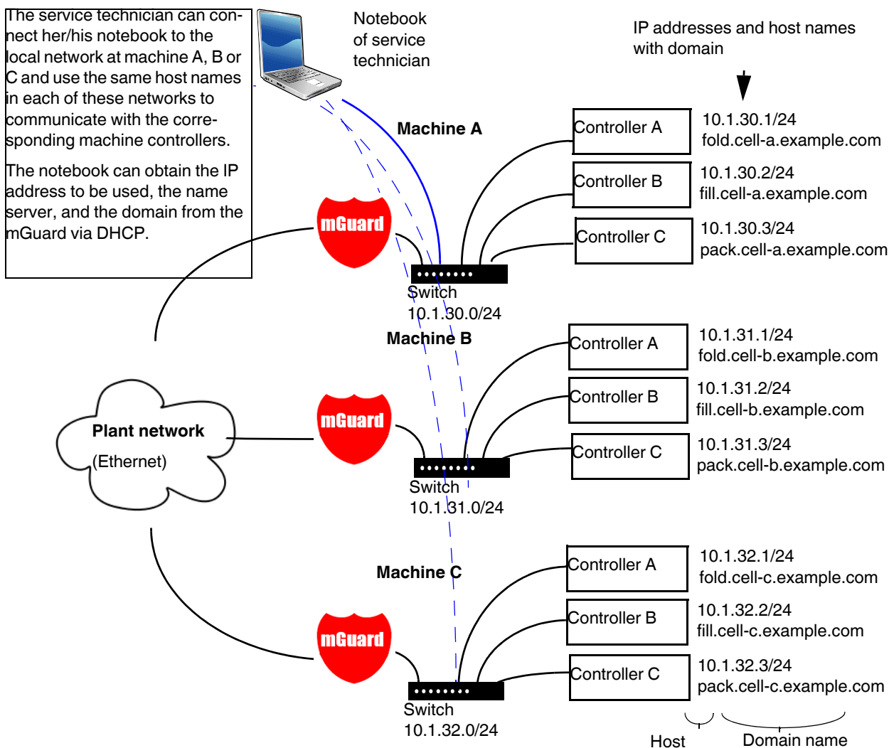
Figure 6-1 Local Resolving of Hostnames
