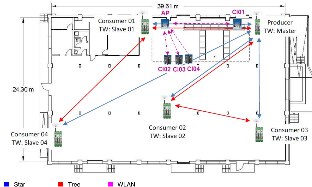
Figure 3 Test set-up
