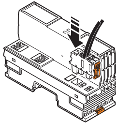
Figure 7-4 Inserting the connector
