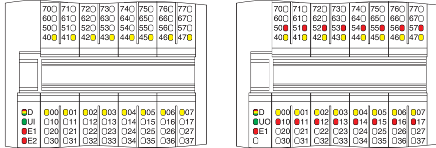
Figure 9-3 LEDs on the I/O connectors (e.g., AXL F DI16/4 2F, AXL F DO16/3 2F)
