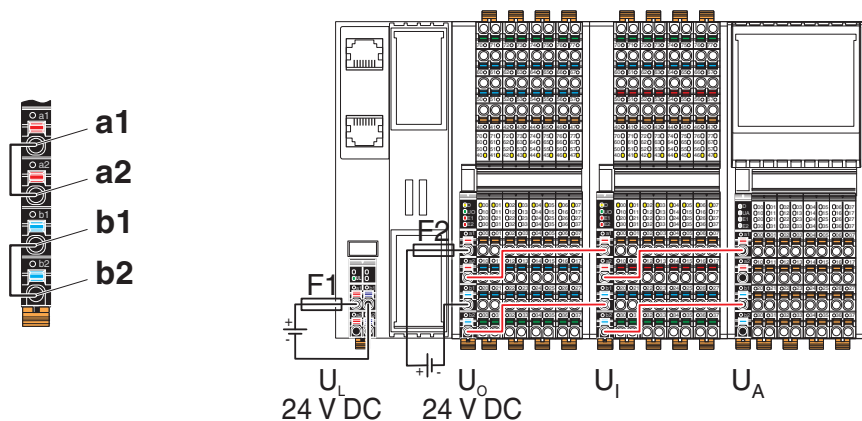
Figure 7-8 Jumpering in the power connector and example of potential forwarding
