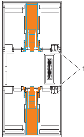
Figure 8-1 FE spring (1)
