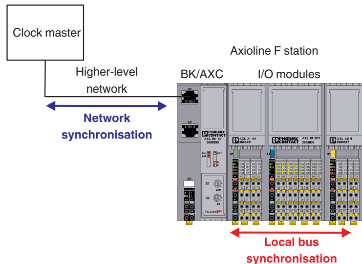
Figure A-3 Network and local bus synchronization
