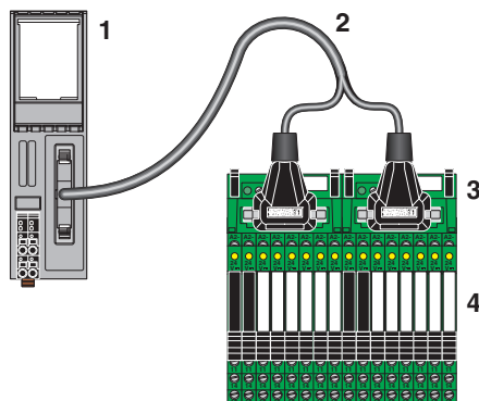
Figure 7-15 Connection of relay modules
