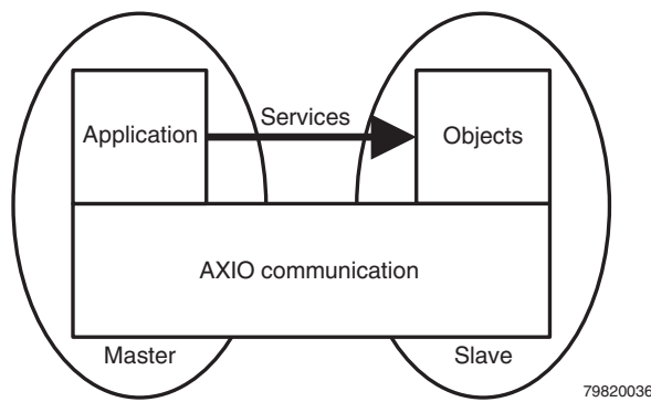
Figure 11-1 PDI components
