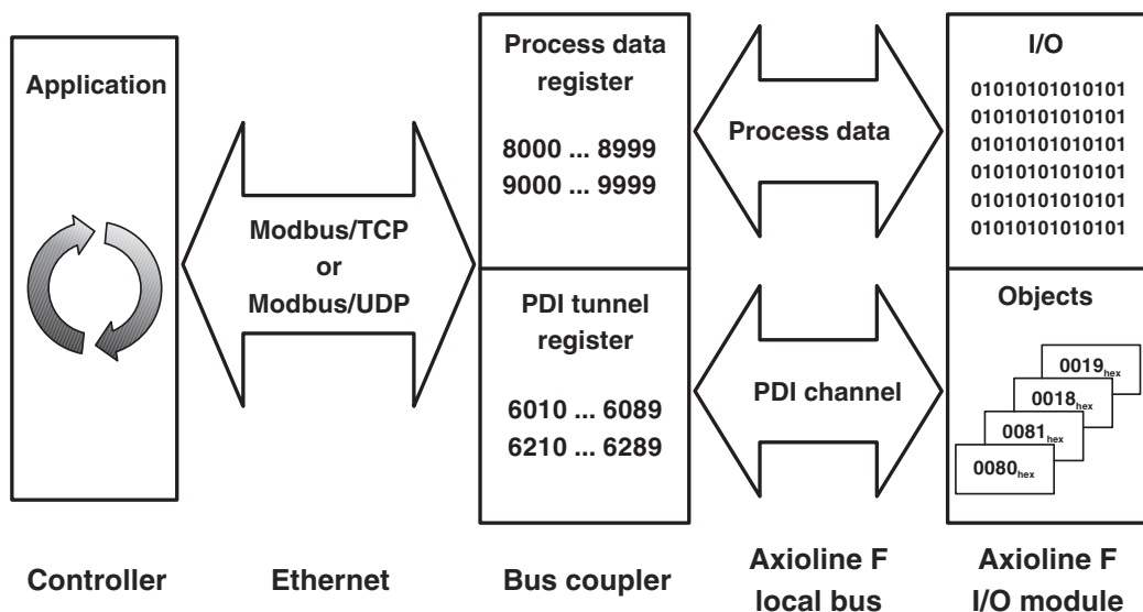
Figure 8 Access to PDI objects
