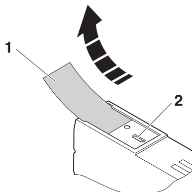
Figure 8 Service interface
