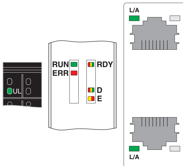
Figure 6 Local diagnostic and status indicators
