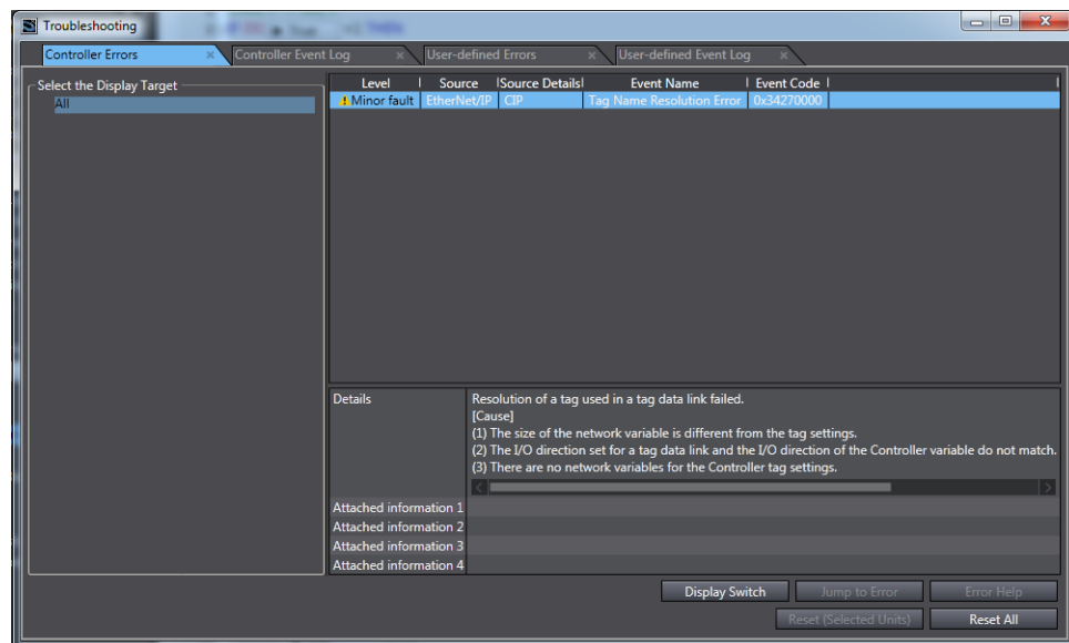
Figure 3-2 Controller errors
