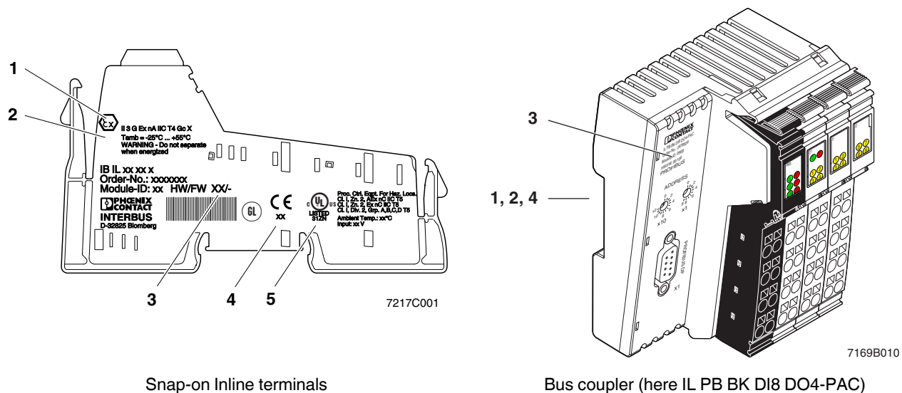
Figure 1 Typical labeling of Inline terminals that are approved for use in zone 2 potentially explosive areas
