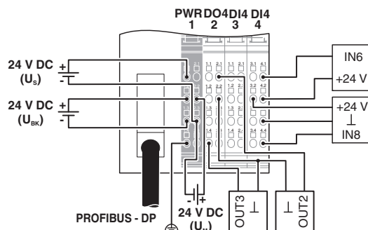
Figure 5 Connection example
