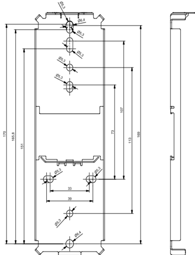
Figure 4-6 Mounting plate
