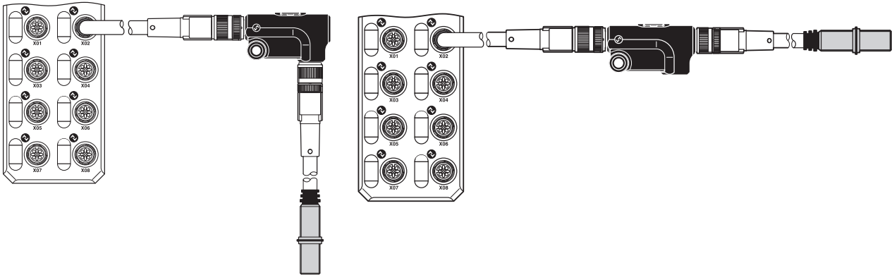
Figure 5-12 Connection of a sensor to an IO-Link master via a rectangular/straight converter
