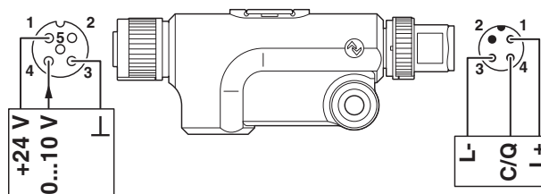
Figure 5 Connection example
