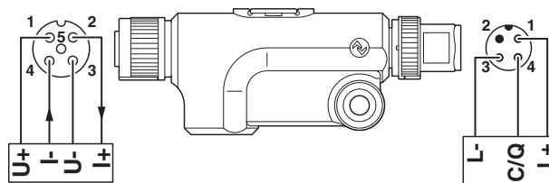
Figure 5 Connection example
