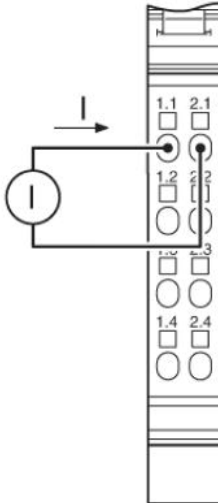
Connection diagram
