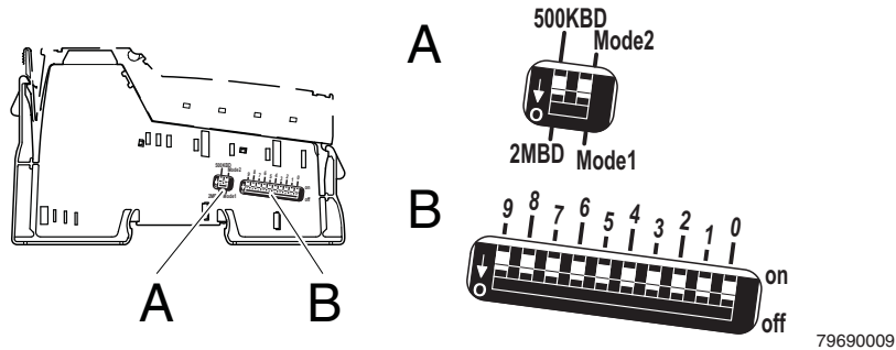
Figure 4-1 DIP switches
