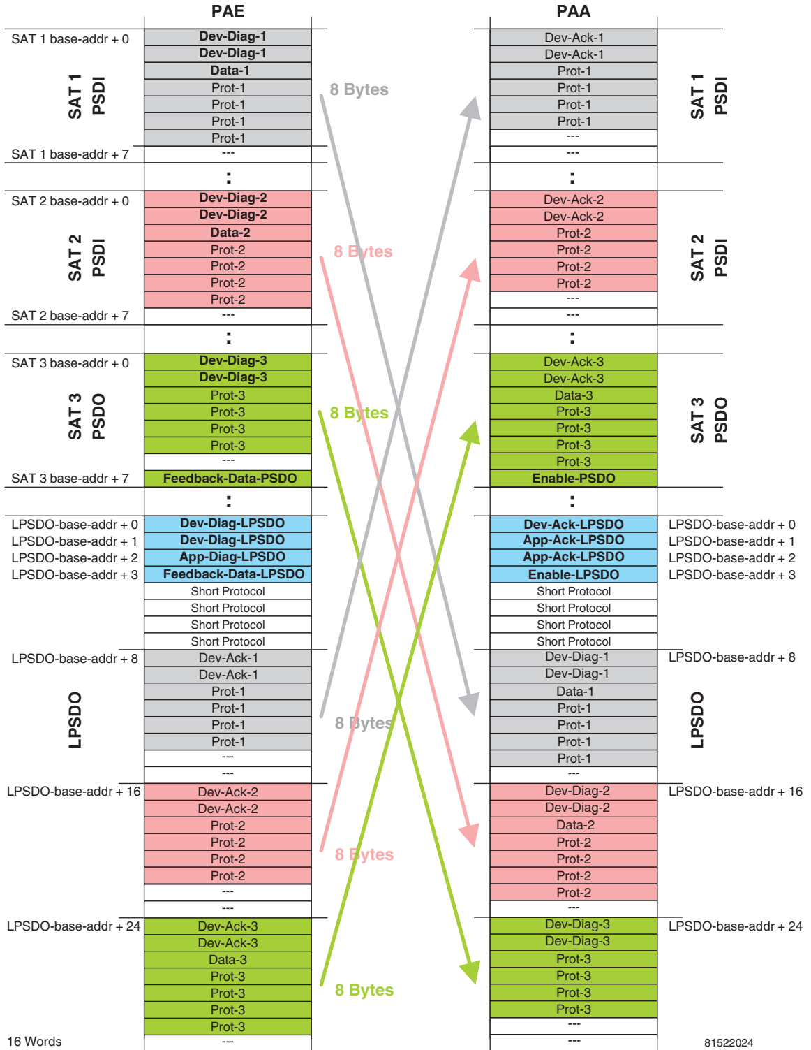
Figure A-4 I/O image and data flow in a system comprising 1 IB IL 24 LPSDO 8 V2-PAC and 3 satellites
