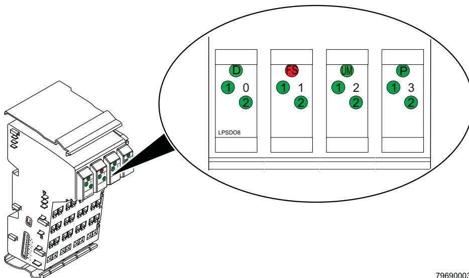
Figure 2-3 Local diagnostic and status indicators of the IB IL 24 LPSDO 8 V2-PAC module
