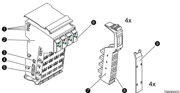
Figure 2-1 Structure of the safety module
