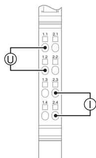
Figure 4 Connection for voltage and current output
