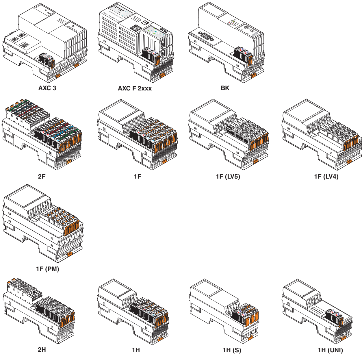
Figure 5-1 Housing versions
