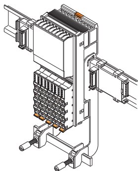
Figure 8-7 Mounting the electronic modules
