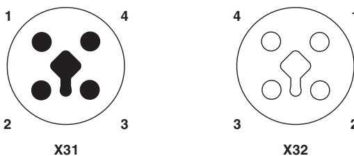
Figure 4 Pin assignment of the power supply, T-coded
