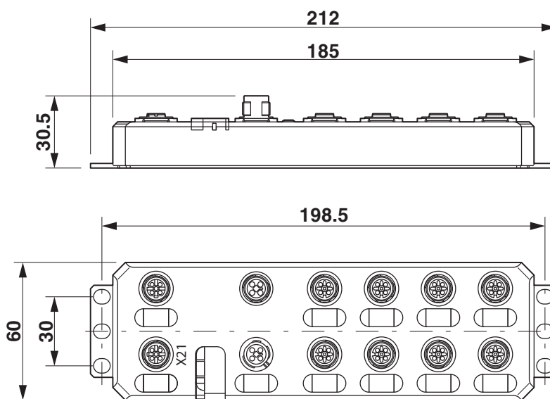
Figure 3-4 Housing dimensions (mm) of metal devices with extended fixing clips
