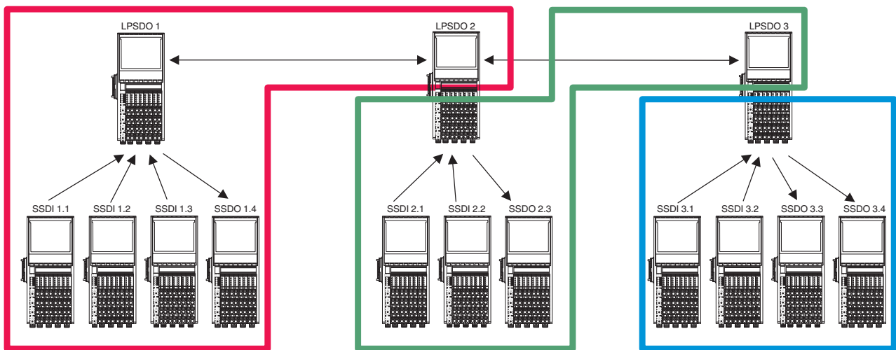
Figure A-7 Flat topology (line structure)
