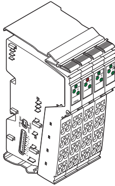
Figure 5-11 Example of a safety module: IB IL 24 PSDO 8-PAC
