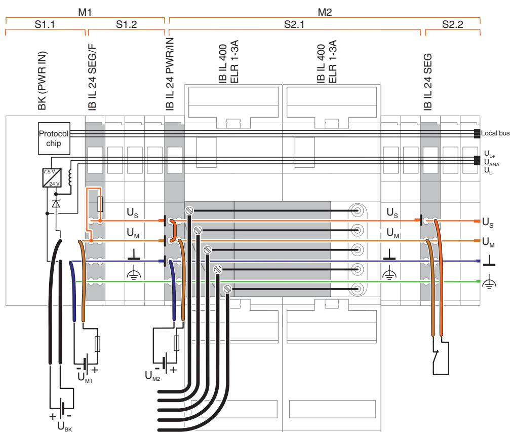
Figure 8-1 Potential routing within an Inline station
