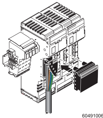
Figure 11-16 Inserting a power bridge
