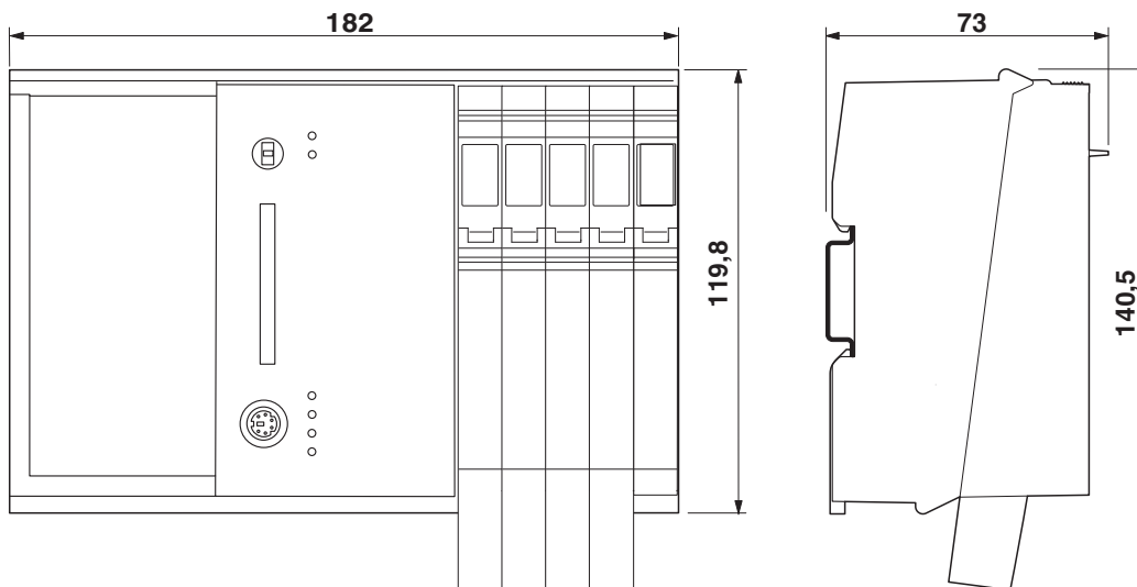
Figure 6-9 Dimensions of container housing 4 (in mm)
