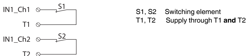
Figure 7-7 Two-channel equivalent assignment of inputs, supply through T1 and T2 (both clocked)
