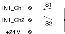
Figure 7-15 Two-channel non-equivalent assignment of inputs, external supply
