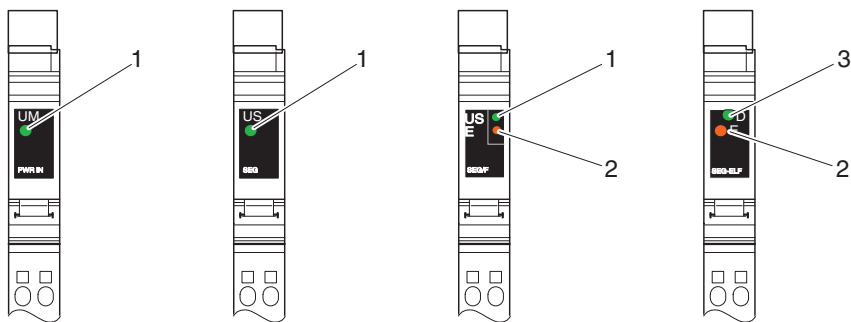
Figure 9-1 Possible indicators on power and segment terminals
