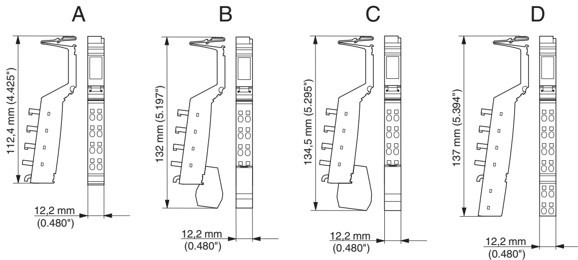
Figure 7-2 Connector dimensions
