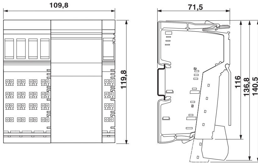
Figure 6-10 Dimensions of container housing 3 (in mm)
