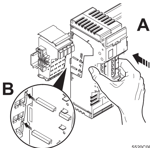
Figure 10-15 Mounting a power-level terminal
