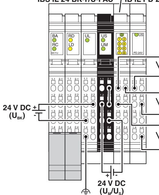
Figure 5 Connection of sensors when using the IB IL PD 24V-PAC terminal
