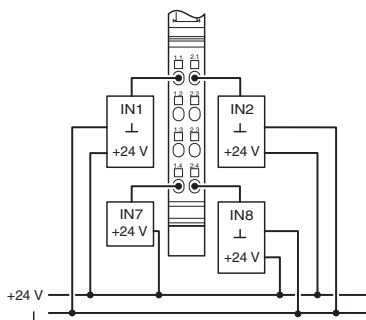
Figure 3 Example of a connection of sensors when using external busbars
