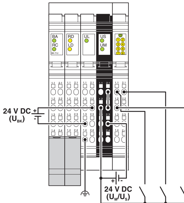
Figure 4 Connection of sensors when using external busbars
