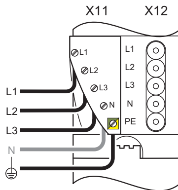
Figure 11-14 Power connector assignment
