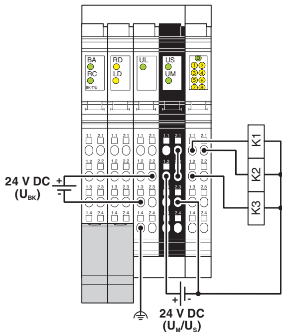
Figure 4 Connection of contactors when using external busbars
