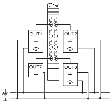
Figure 3 Typical connection of actuators when using external busbars
