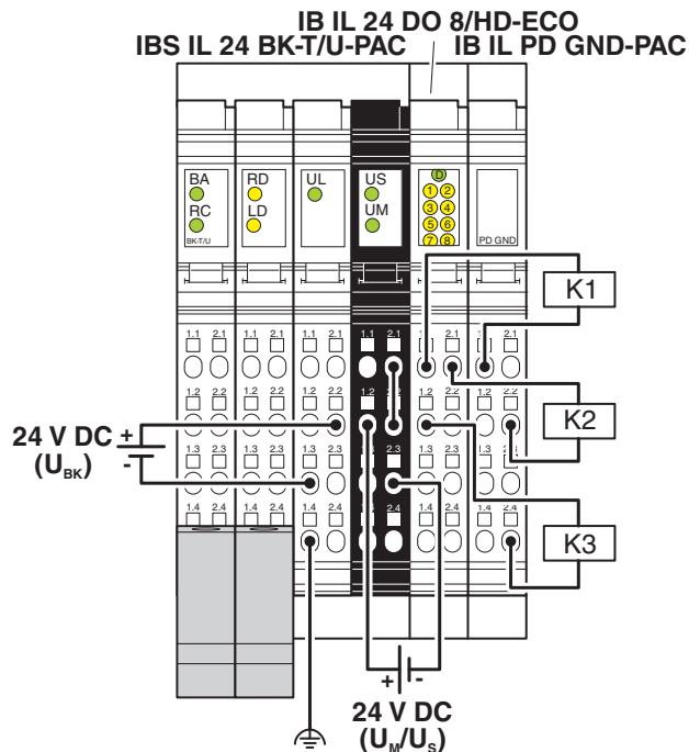
Figure 5 Connection of contactors when using the IB IL PD GND-PAC terminal
