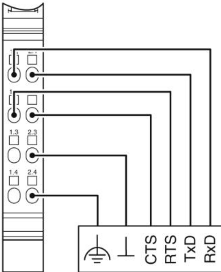
RS-232 interface wiring: four-wire handshake
