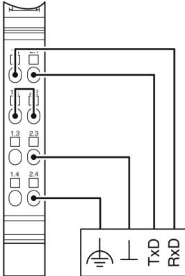
Connection diagram
