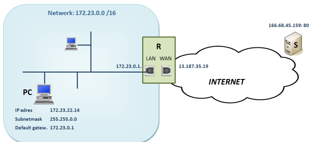
Figure 6.3: Linking of a private network to the Internet via a router
