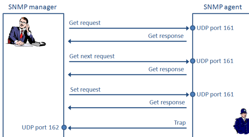
Figure 4.12: SNMP communication
