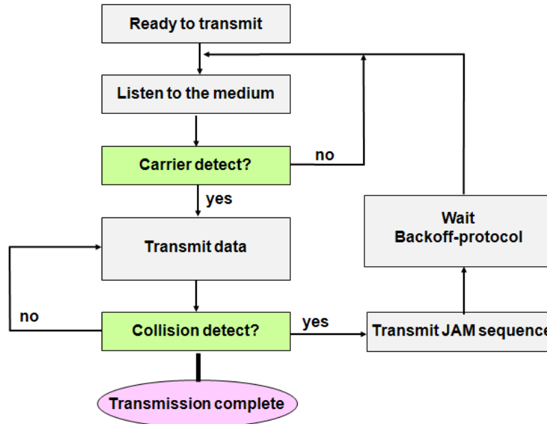
Figure 2.13: CSMA/CD flow
