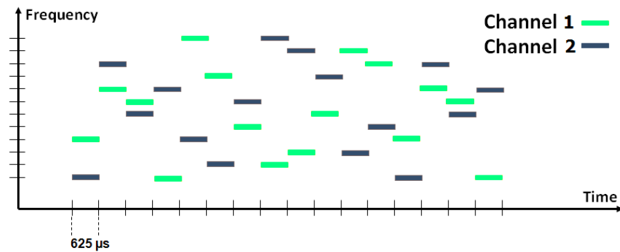
Figure 2.7: FHSS technology
