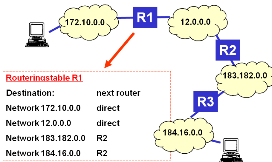
Figure 3.6: Functioning router
