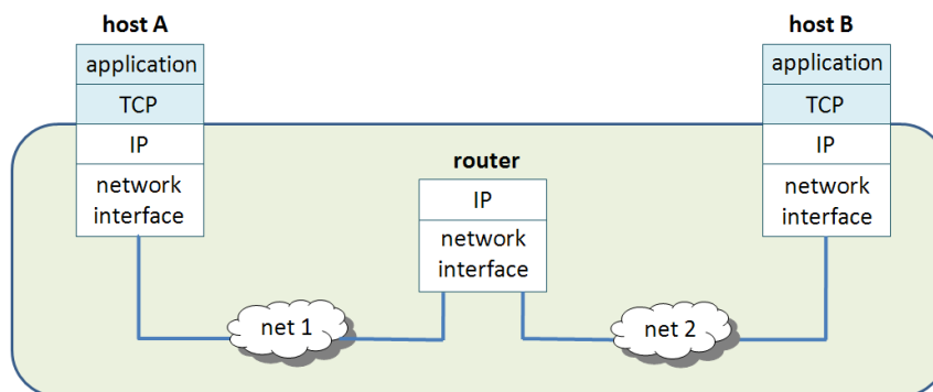
Figure 3.10: TCP is end-to-end transport protocol
