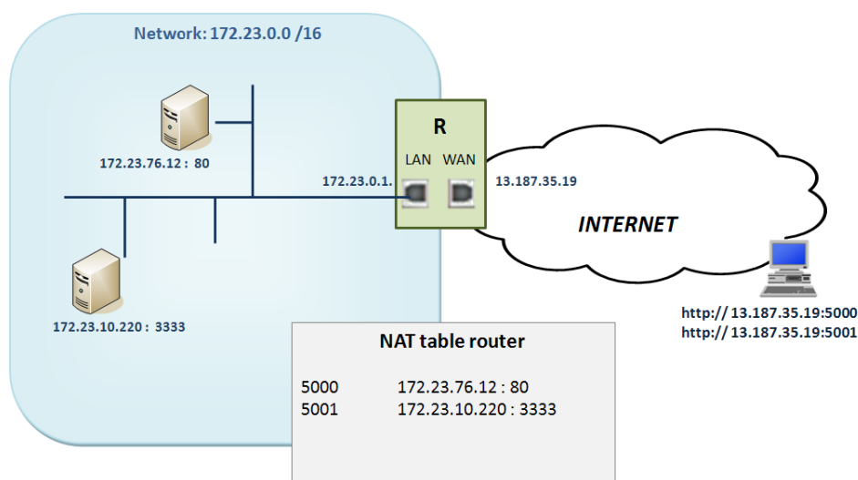
Figure 6.6: Port forwarding
