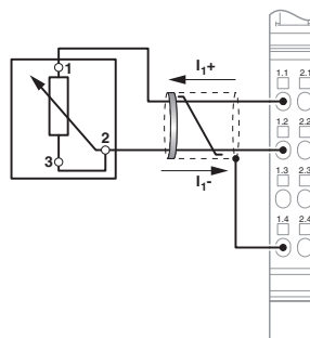
Figure 6 Connection of a potentiometer in 2-wire technology with shield connection
