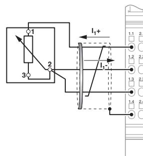
Figure 7 Connection of a potentiometer in 3-wire technology with shield connection
