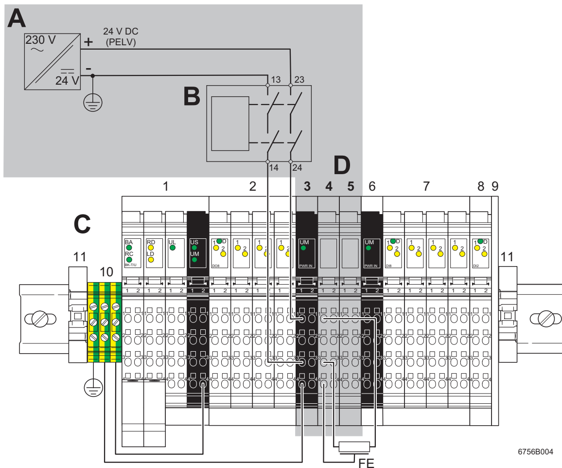
Figure 4 Typical connection of the supply voltage
