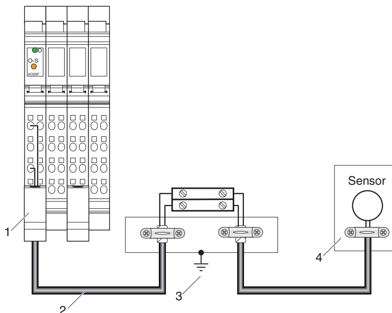
Figure 10-11 Integration of analog shielding in a concept with central equipotential bonding at the control cabinet entry
