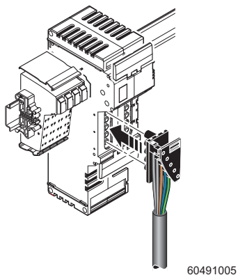
Figure 11-15 Connecting a power connector
