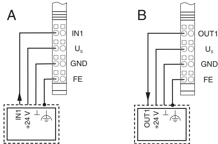
Figure 11-11 4-wire termination for digital devices
