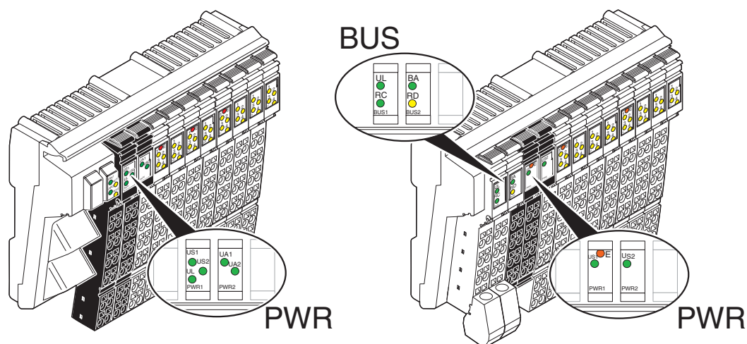
Figure 9-6 Possible indicators in the supply function area
