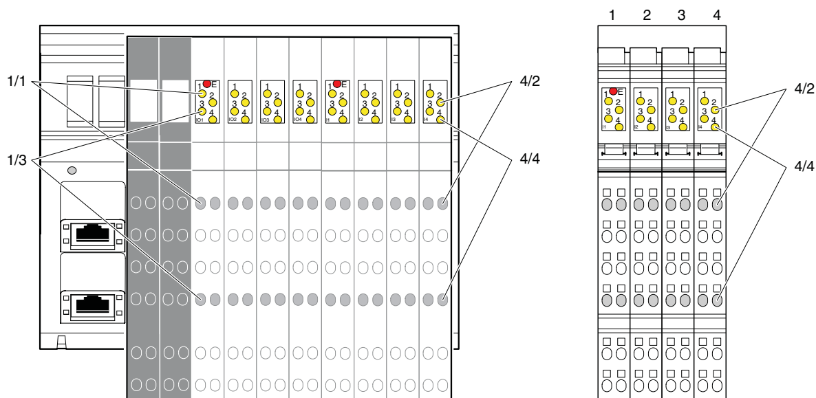
Figure 9-8 Assignment between status LED and input/output
