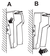
Figure 10-17 Snapping on the base
