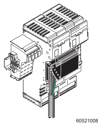
Figure 11-17 Power-level terminals with a mains connector and power bridge
