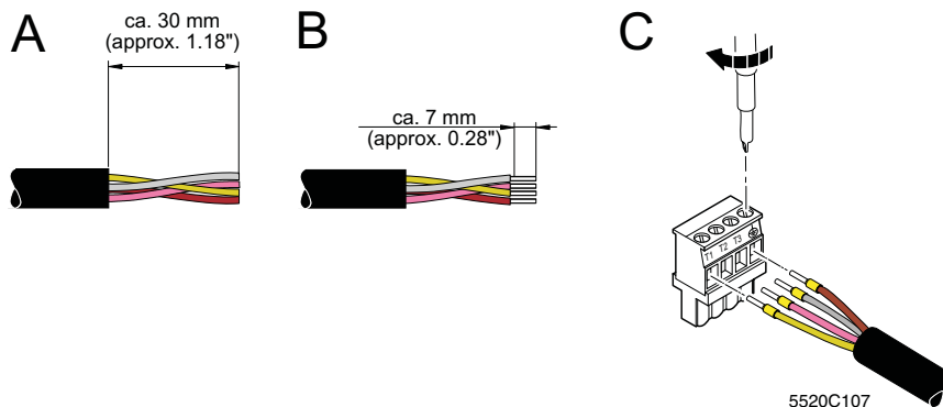
Figure 11-18 Assembling the motor circuit connector
