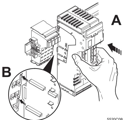
Figure 10-15 Mounting a power-level terminal
