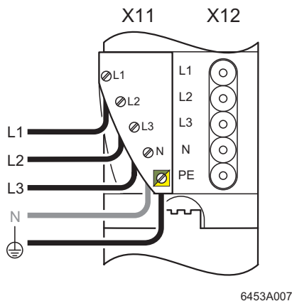
Figure 11-14 Power connector assignment
