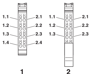
Figure 2 Terminal point assignment
