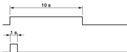
Figure 7 Two single shots with different lengths
