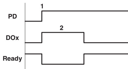
Figure 8 Pulse generation sequence following specification of a time basis and/or factor
