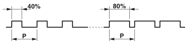
Figure 5 PWM with constant period (P) and variable duty cycle of 40 % or 80 %
