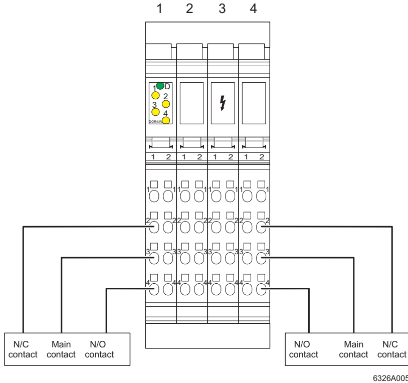
Figure 4 Typical connection of actuators
