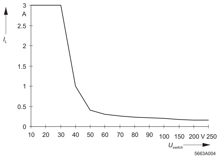
Load Current ( I_L in A) as a Function of the Switching Voltage ( U_{\text{switch}} in V)
