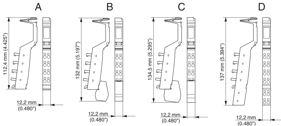
Figure 7-2 Connector dimensions
