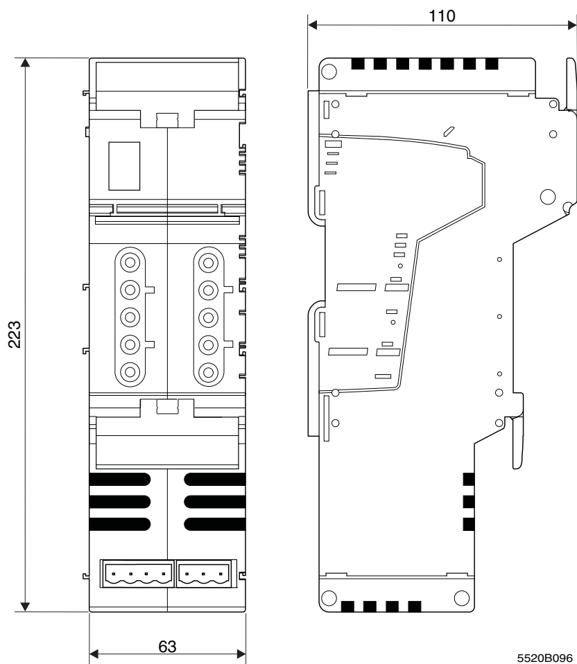
Figure 6-13 Dimensions of power housing
