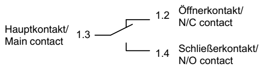
Figure 8 Output relay contacts
